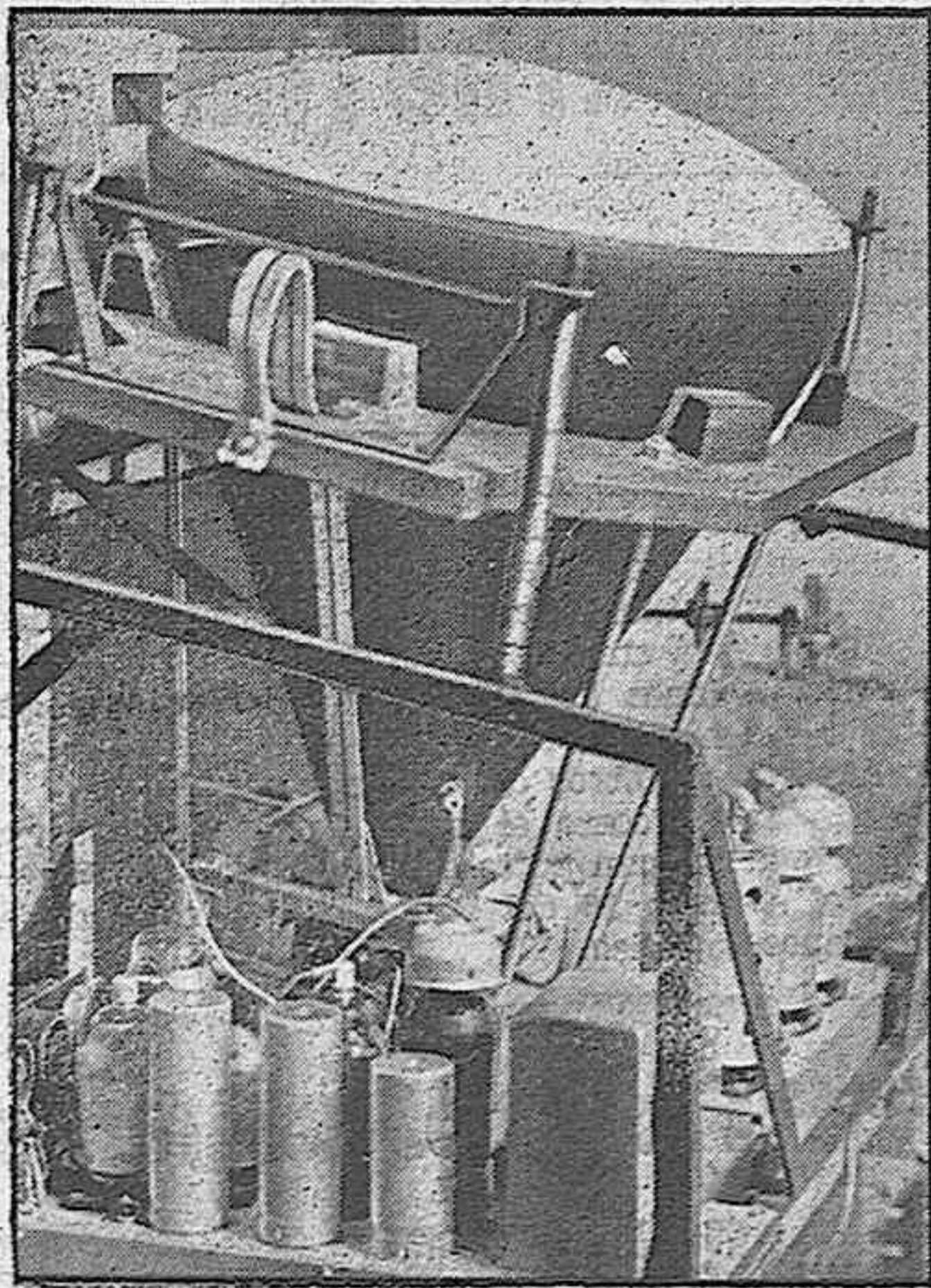
VISTA DEL INTERIOR DEL RECEPTOR DE TELEVISION TELEFUNKEN
