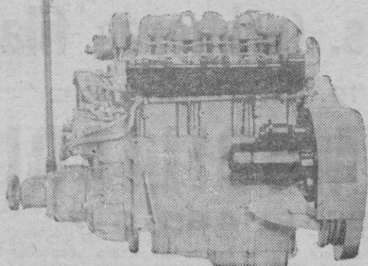
Volvo Penta 3-cylinder 4-stroke diesel engine with direct injection 35 h.p.
