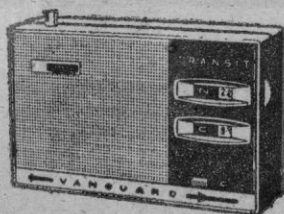
TRANSIT
