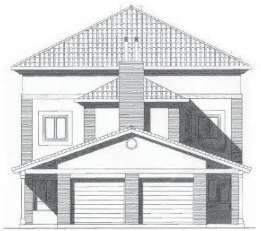
ALZADO PRINCIPAL
