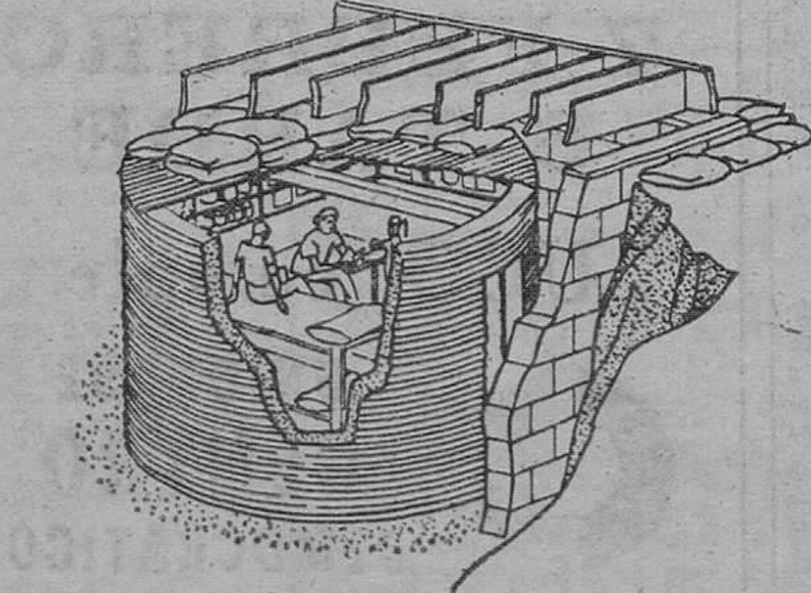
FIGURA 2. MOD. CIRCULOS CONCENTRICOS
