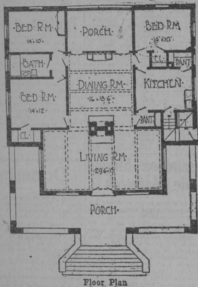
Floor Plan
