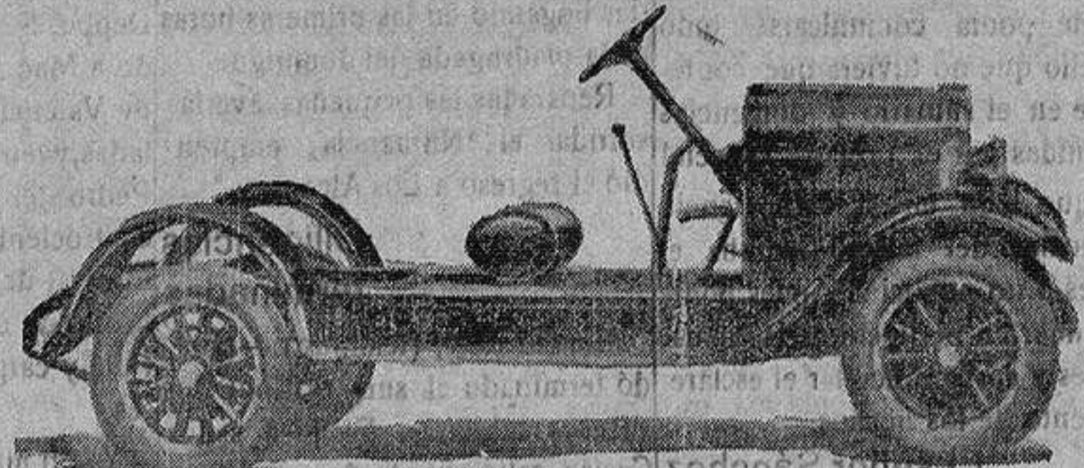
CHASSIS COMERCIAL "RUGBY" 4 CILINDROS
