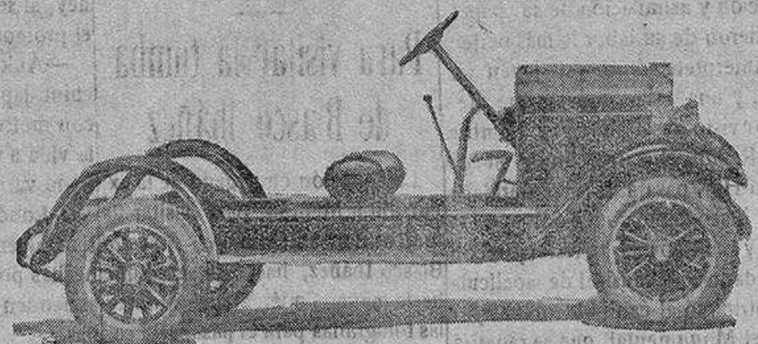
CHASSIS COMERCIAL "RUGBY" 4 CILINDROS
