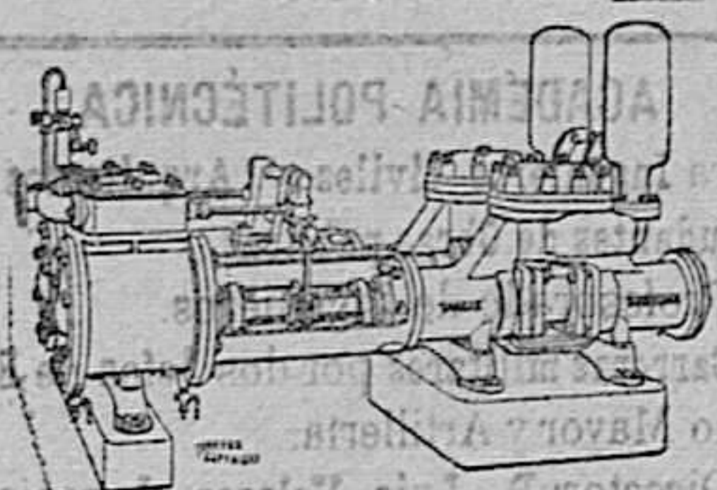
Bomba "Tangyes"
