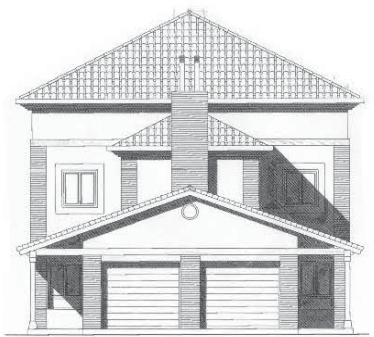
ALZADO PRINCIPAL
