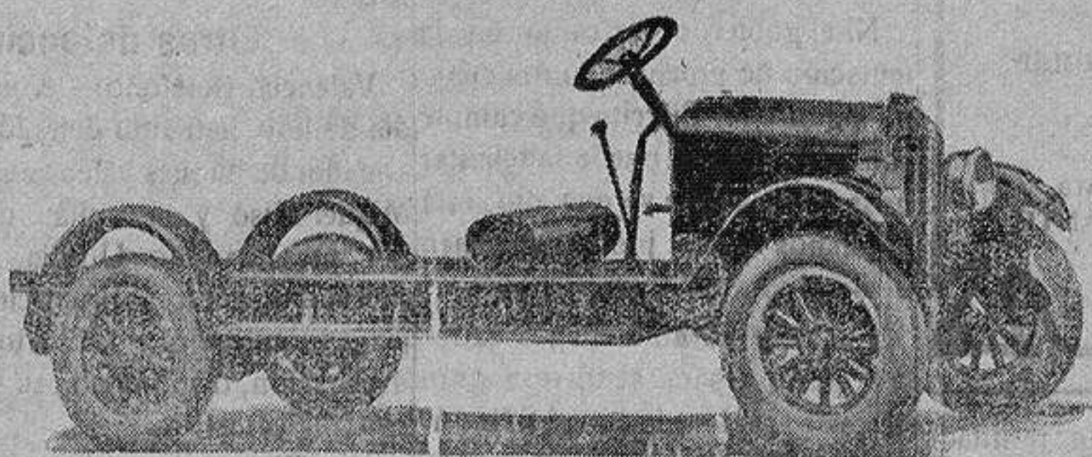
CHASSIS "RUGBY," 4 CILINDROS 1½ y 1¼ TONELADAS
